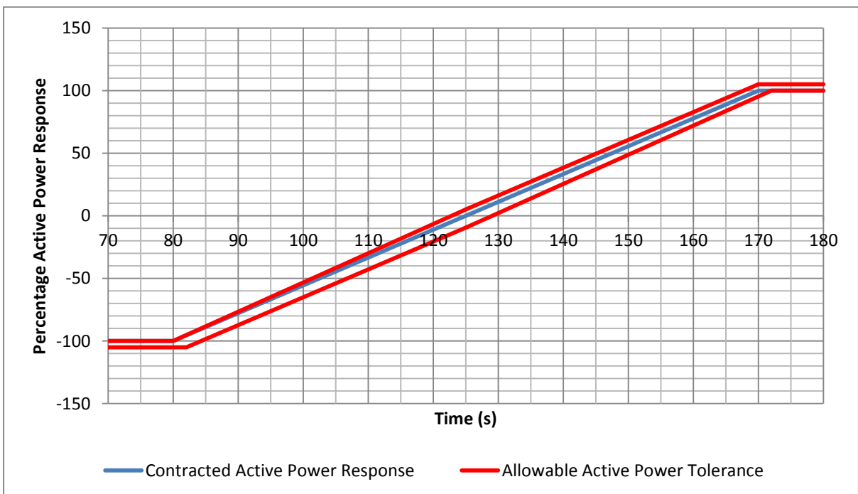
Figure 3.11 - Positive Active Power Gradient Tolerance Band
