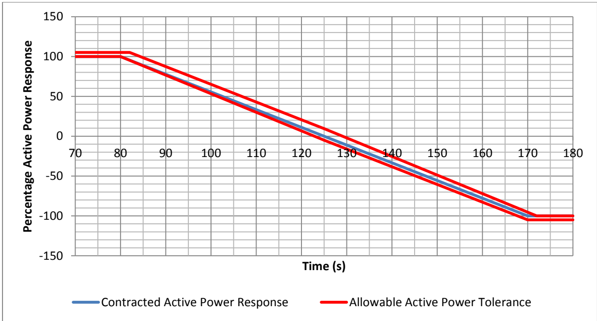
Figure 3.10 - Negative Active Power Gradient Tolerance Band
