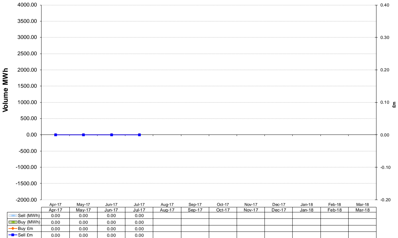
PGBT Actions
