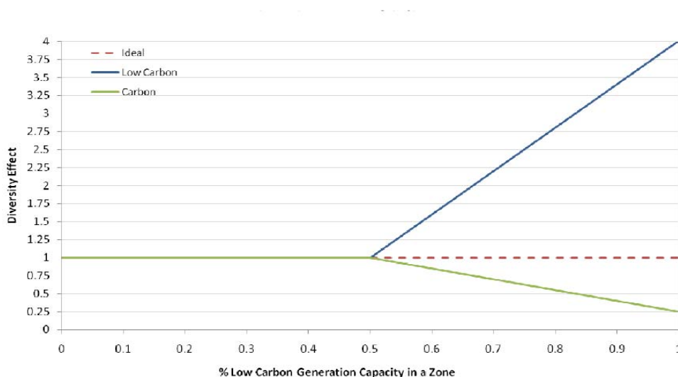
Figure 12 – Normalised effect of Load Factor with changing percentage generation mix in a zone
