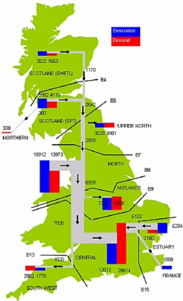
Figure 4.1 - ACS Power Flow Pattern for 2008/09
