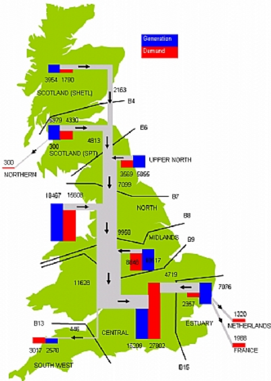
Figure 4.2 - ACS Power Flow Pattern for 2014/15
