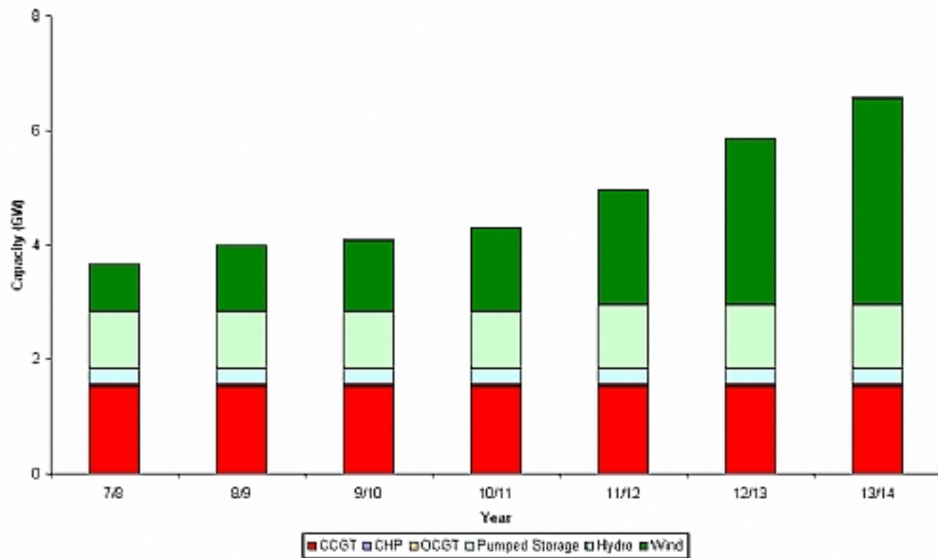
Figure 3.3b - Plant Type by Zone (SHETL), 2007/08 to 2013/14
