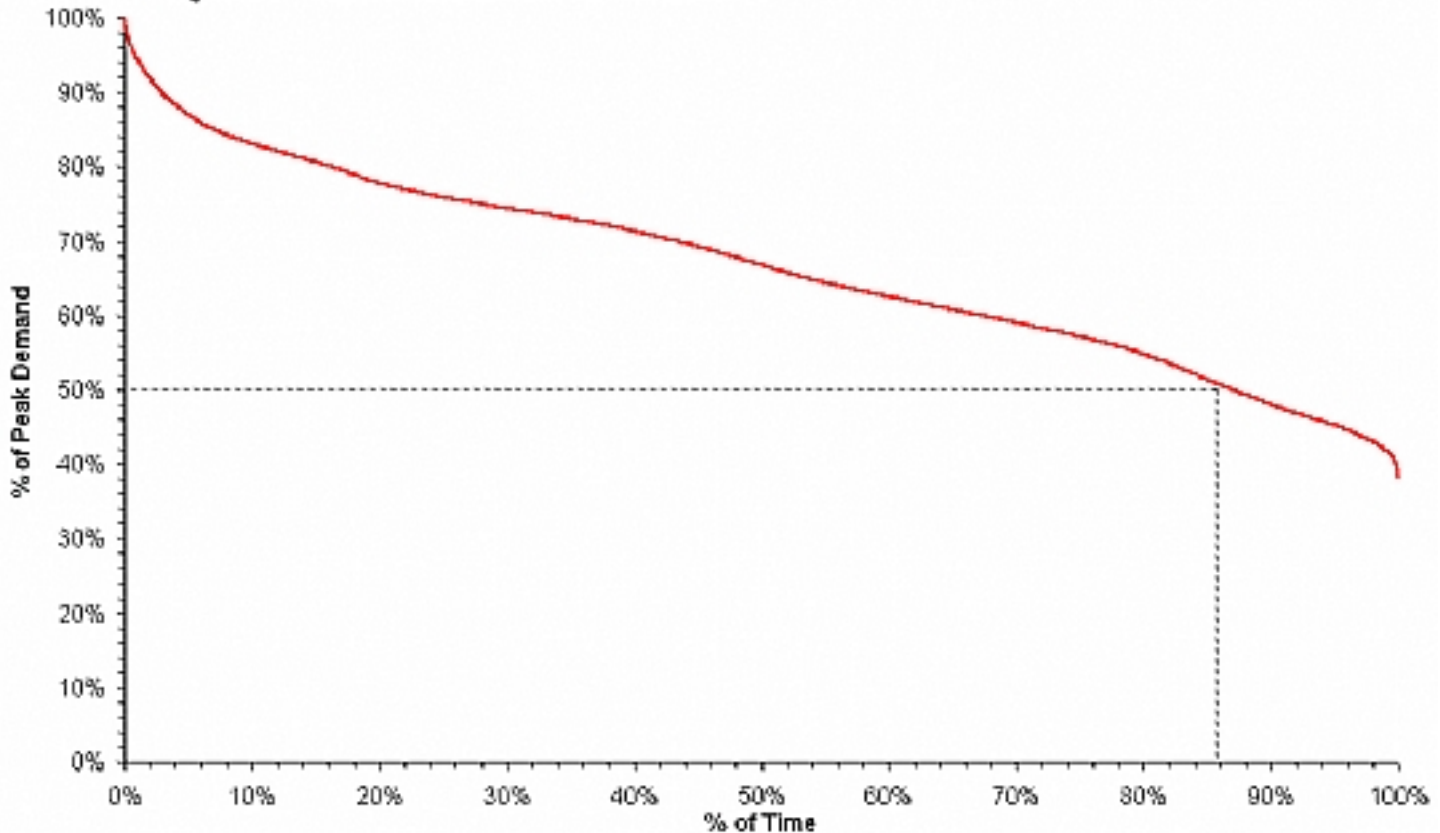
Figure 2.4 - GB Annual Load Duration Curve for 2006/07
