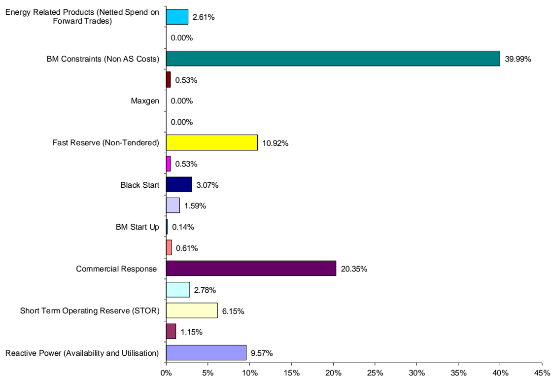
Summary of Balancing Services Costs February 2016
