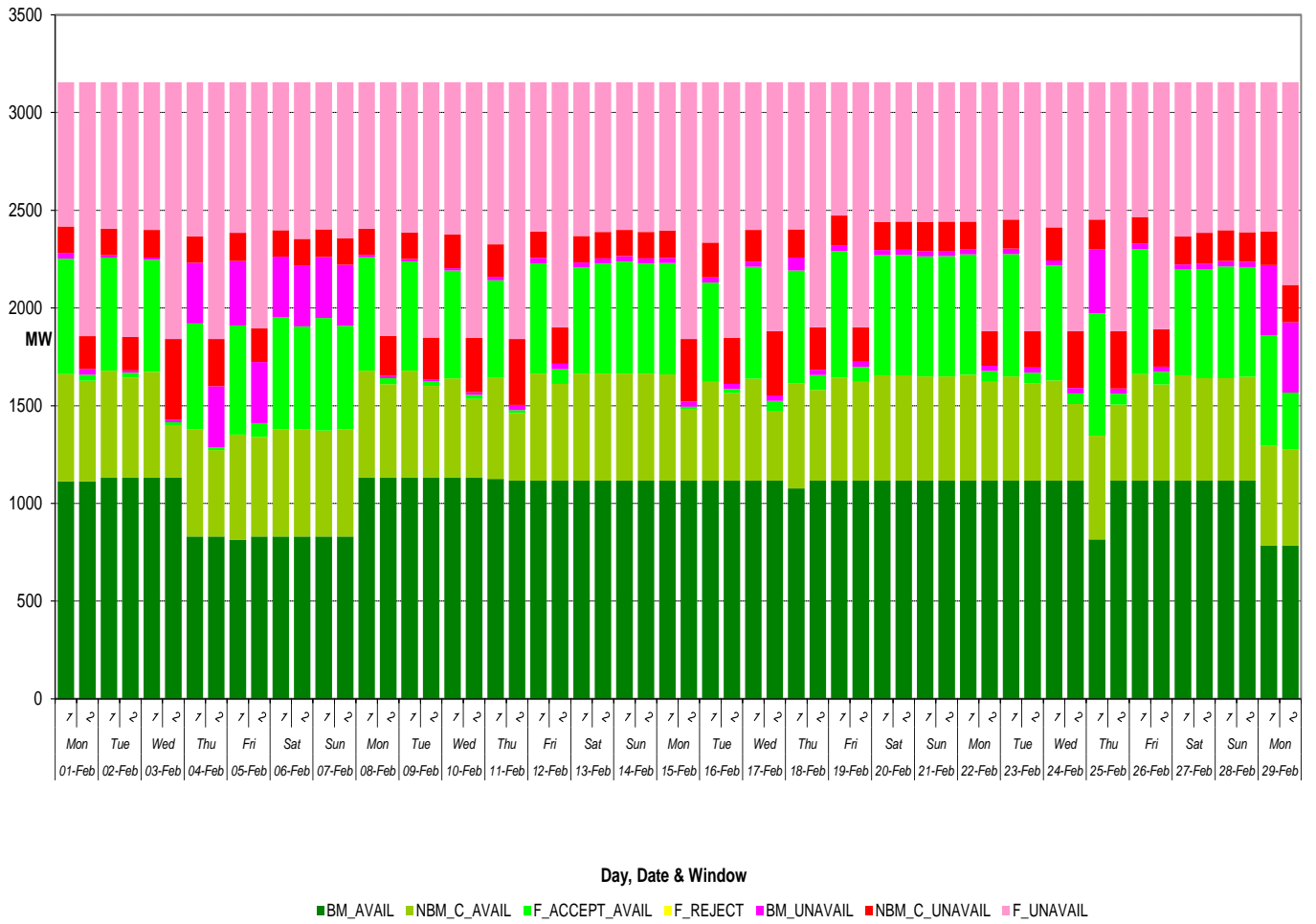
STOR MW Profile for month of Feb 2016
