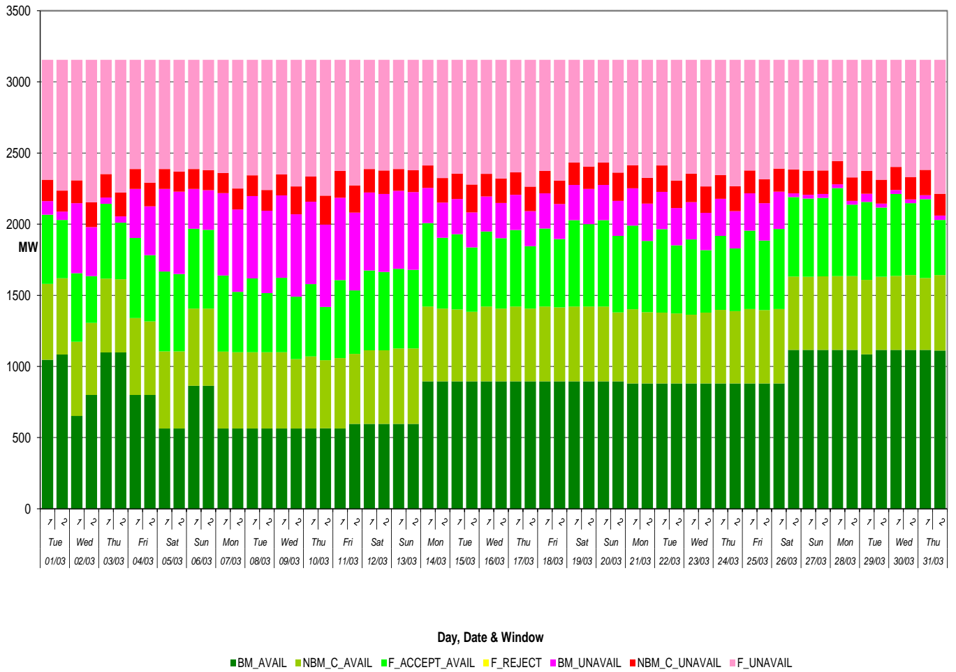
STOR MW Profile for month of Mar 2016
