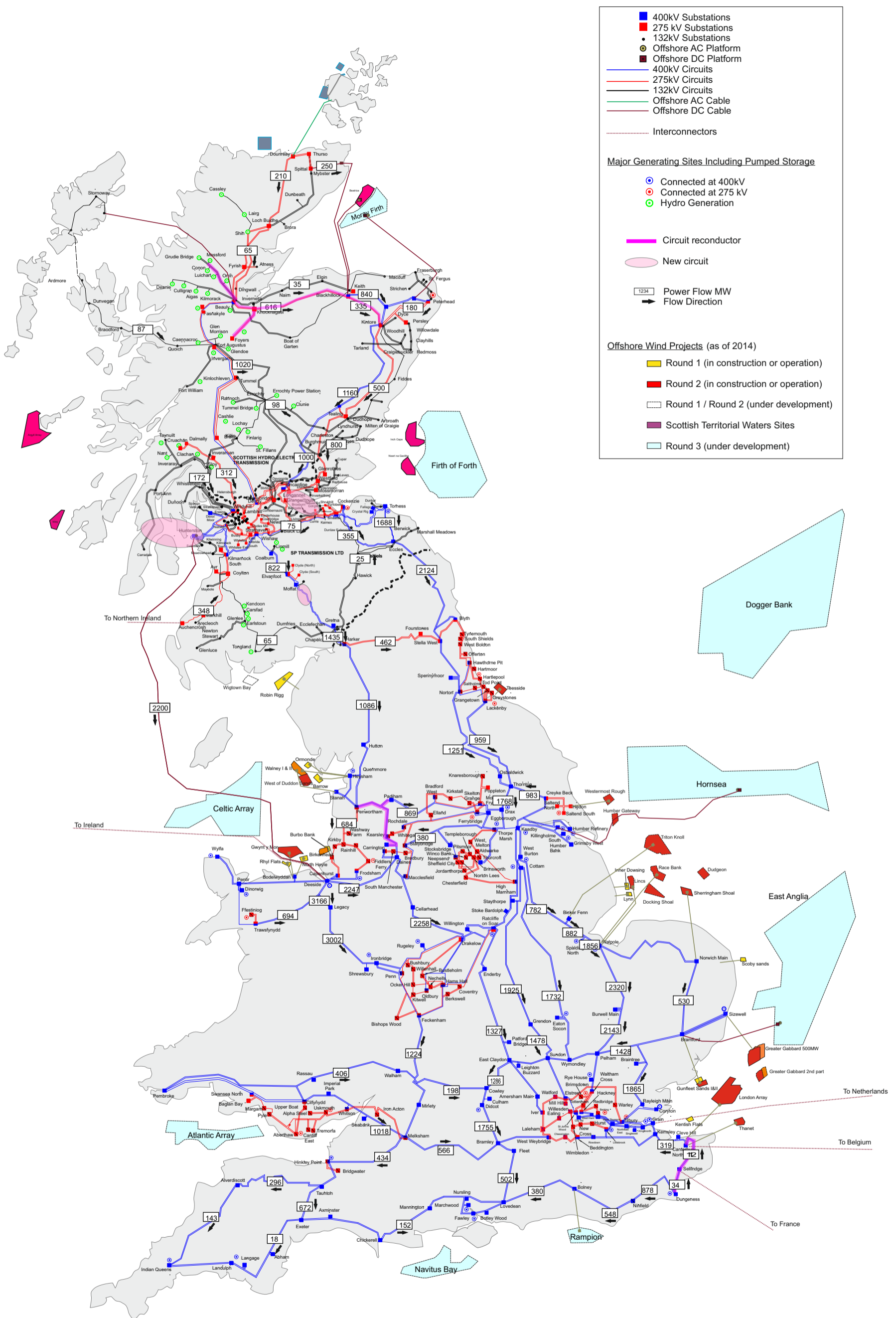
Figure C1.4: GB Power Flow Diagram Gone Green 2020/21
