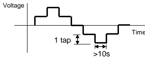
OC5.A.3.8 Figure 1 – T transformer tap sequence for reactive transfer tests
