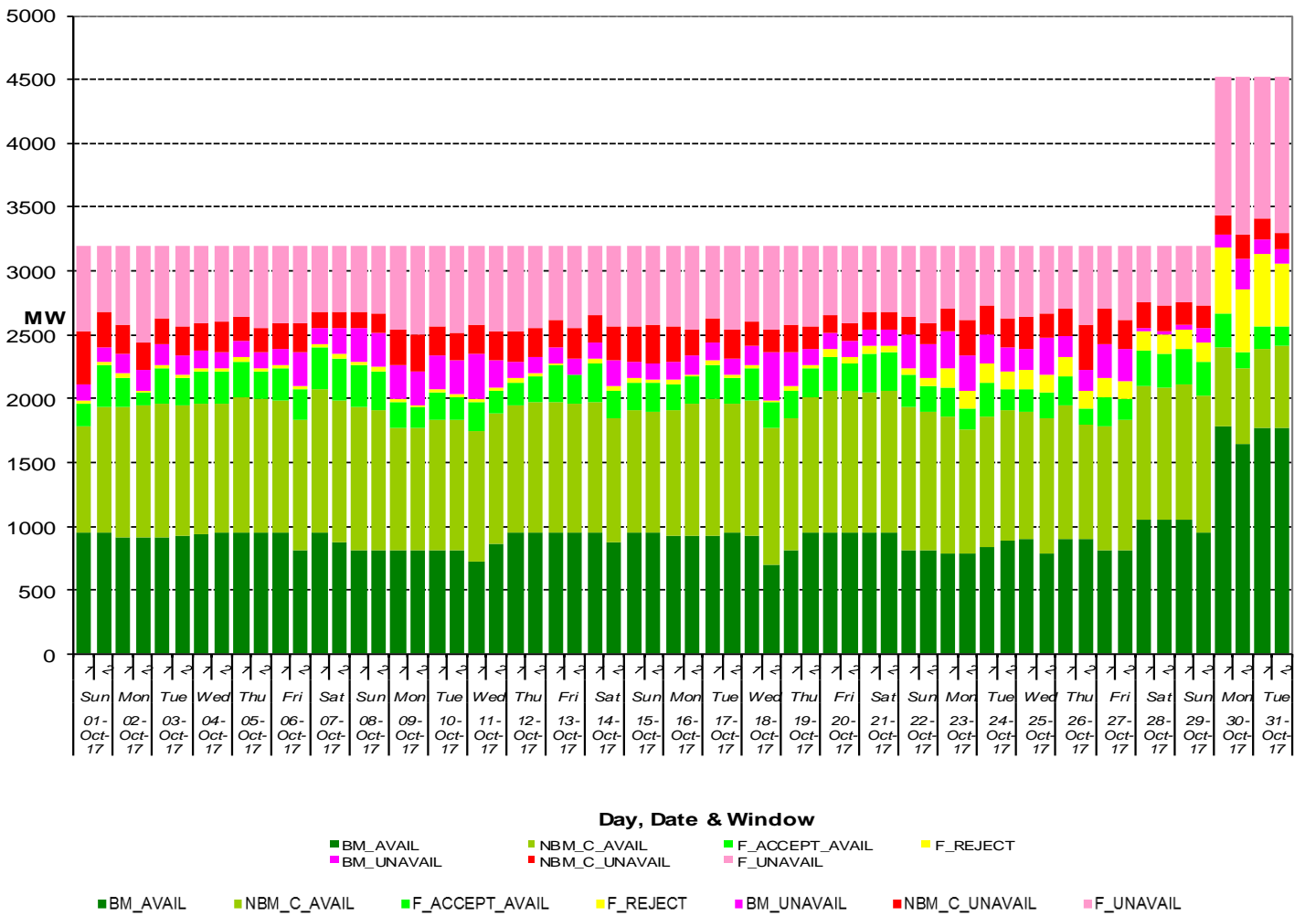
STOR MW Profile for month of Oct 2017
